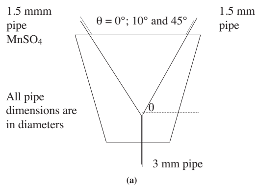
Figure 1—(a) Reagent feed configuration in the presence of micromixing; (b) The actual micromixing device
